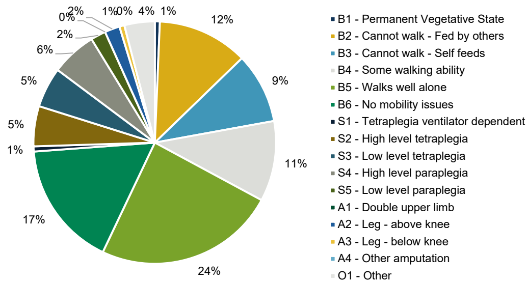
Figure P.4: Detailed split of the number of Motor (non-MIB) PPO claims, by IFoA PPO Working Party injury type categorisation
