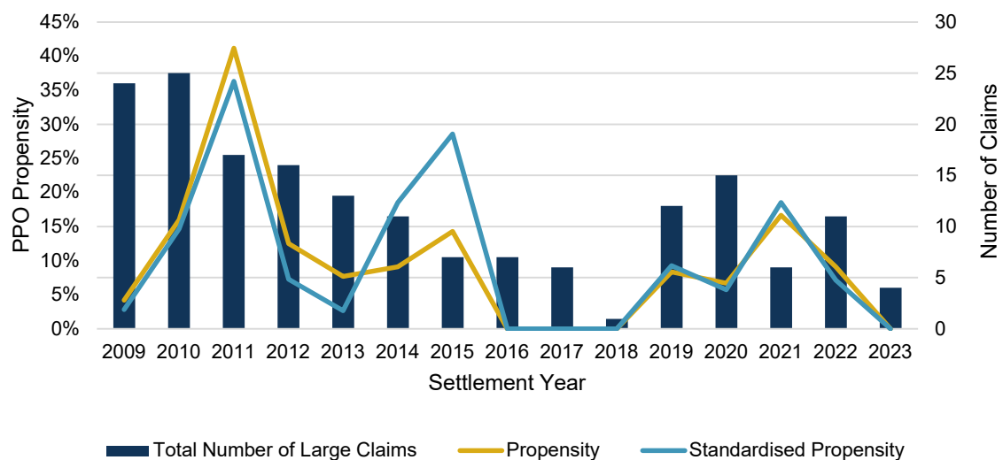
Figure H.4: Liability PPO propensity and standardised Liability PPO propensity, by settlement year, with Ogden adjustment
