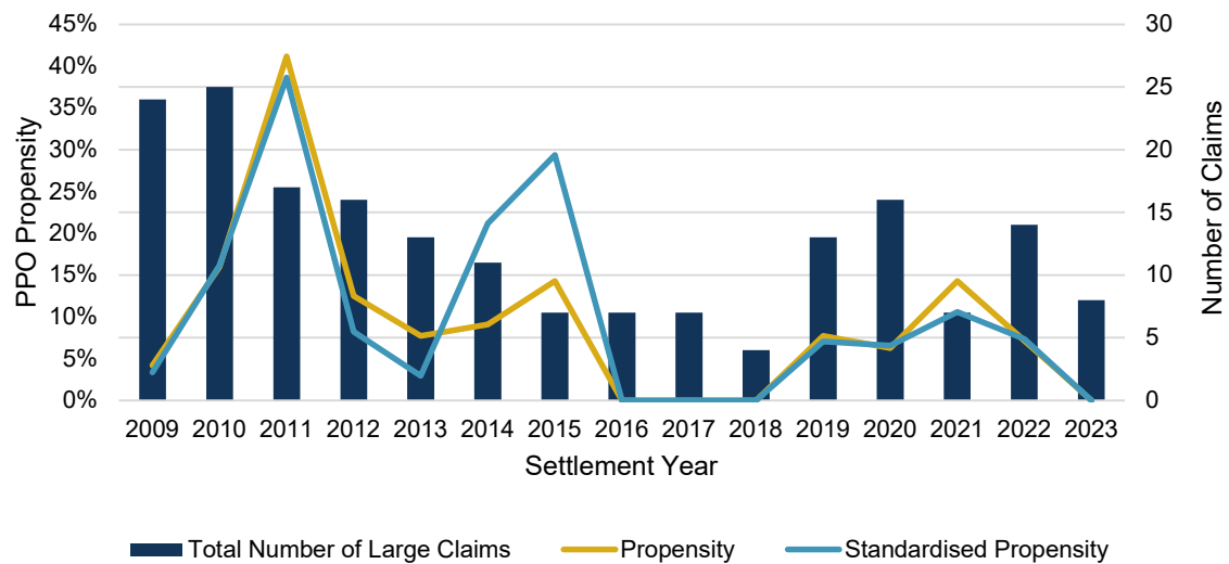
Figure H.3: Liability PPO propensity and standardised Liability PPO propensity, by settlement year
