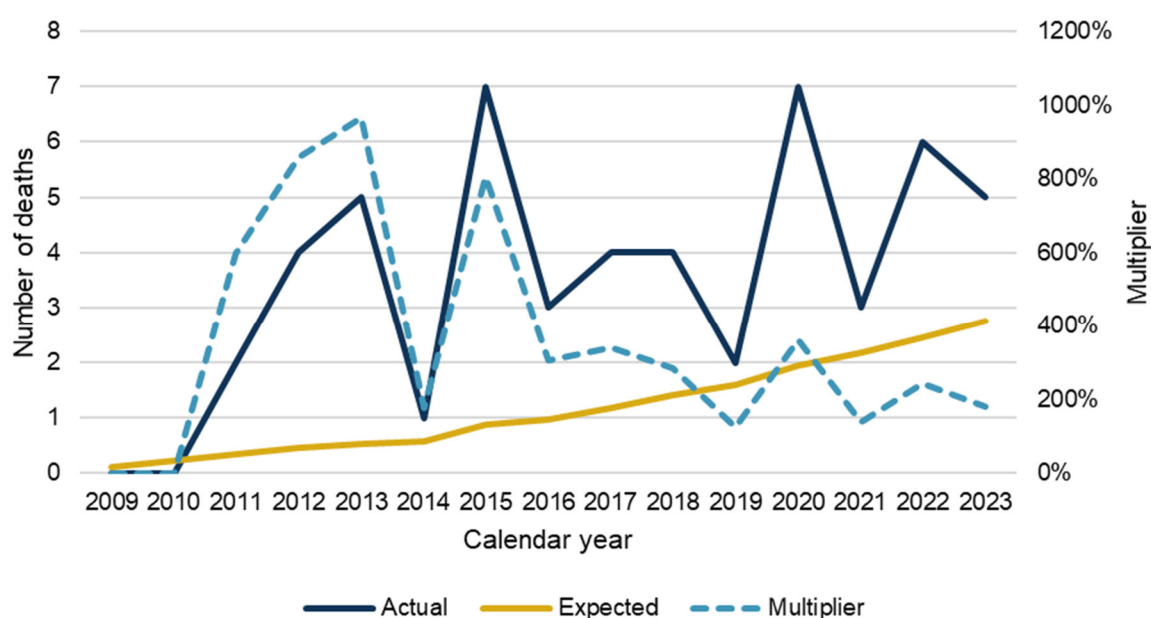
Figure 39: Actual number of PPO claimant deaths, expected number of PPO claimant deaths assuming unimpaired mortality, and the multiplier (actual / expected), by calendar year
