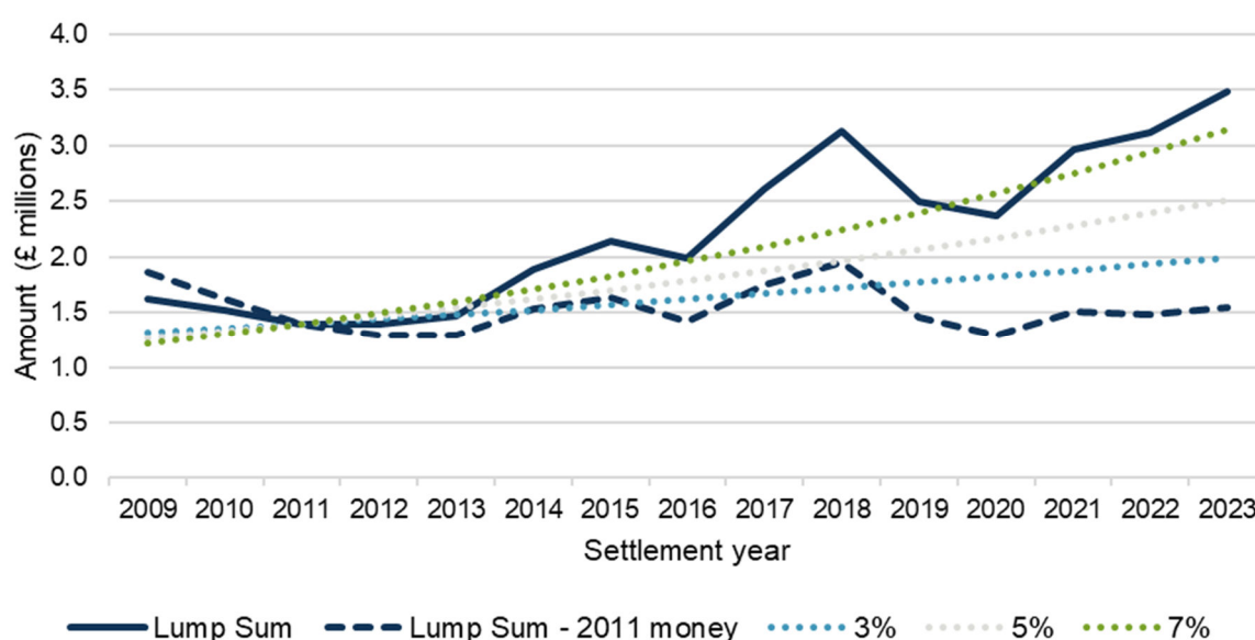
Figure 29: Average size of the lump sum element of Motor (non-MIB) PPO claims, nominal and with inflation removed (assuming inflation of 7% per annum), by settlement year
