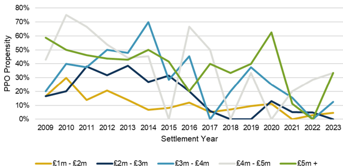
Figure 13: Motor (non-MIB) PPO propensity, by incremental large claim threshold band (2011 terms), and by settlement year
