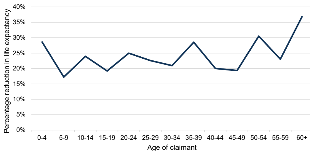
Figure J.29: Distribution of the percentage reduction in life expectancy of a claimant, for Motor (non-MIB) PPO claims, by age of claimant at accident date, for claims settled since 2009
