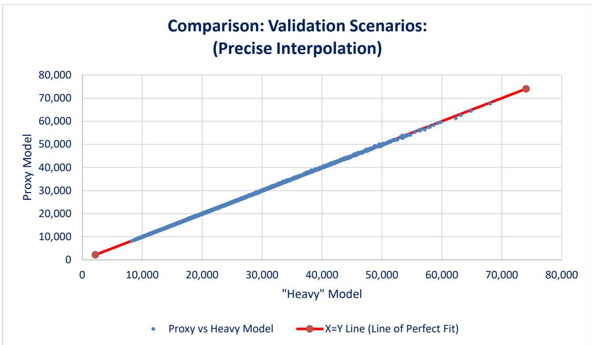
Figure 9: comparison of validation scenarios under precise interpolation approach
