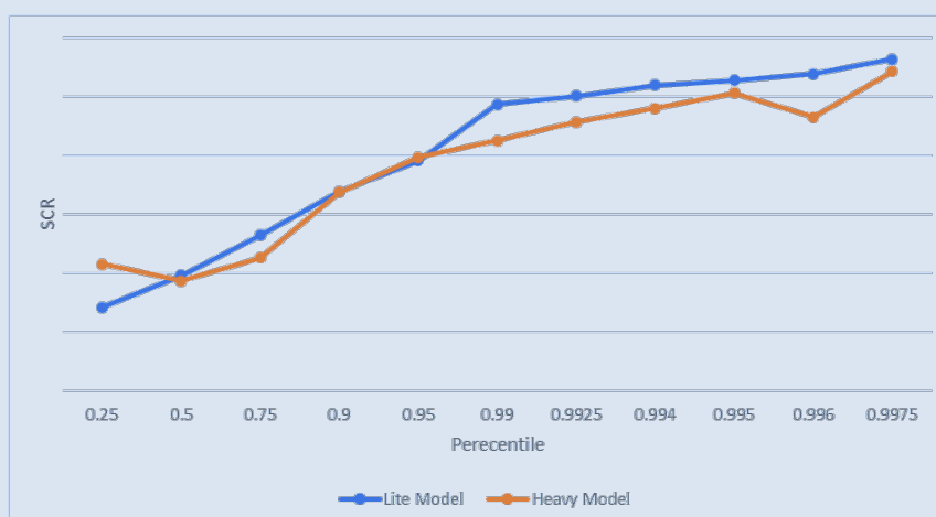
Figure 21: results of ranking test
