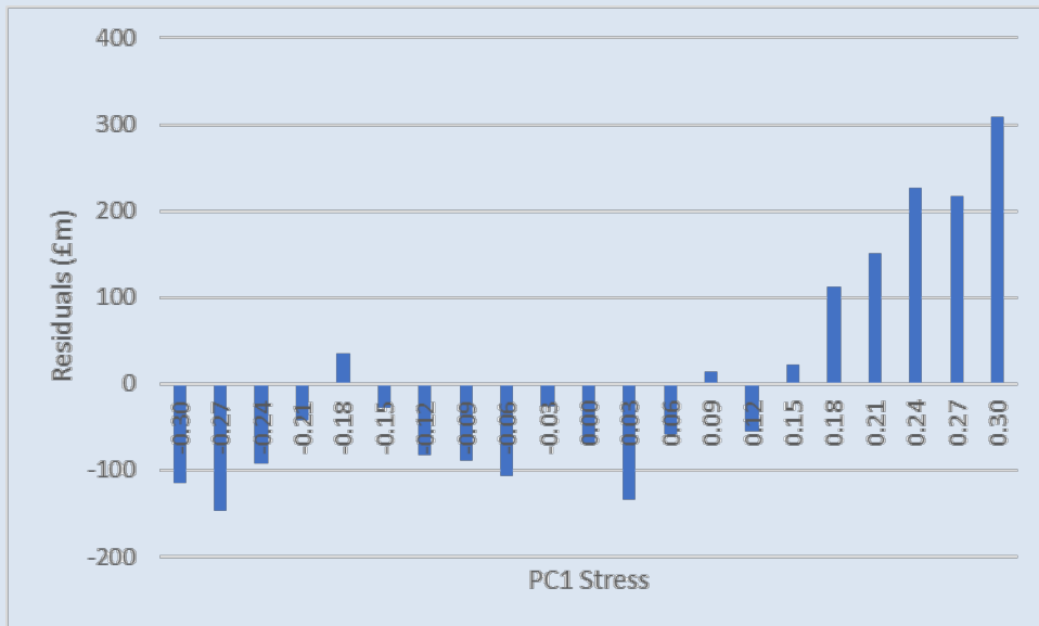
Figure 20: plotted residuals of bias test following increase in terms
