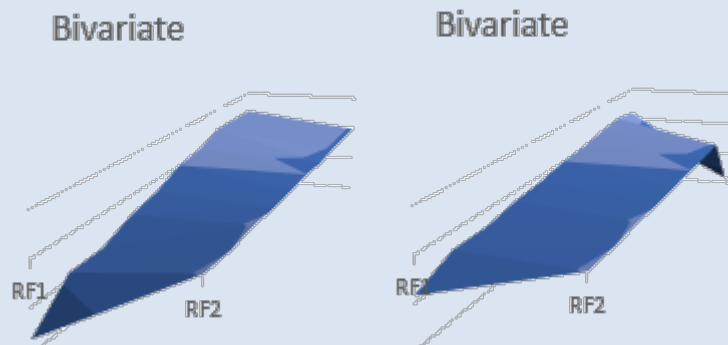
Figure 24: graphical analysis of risk factors
