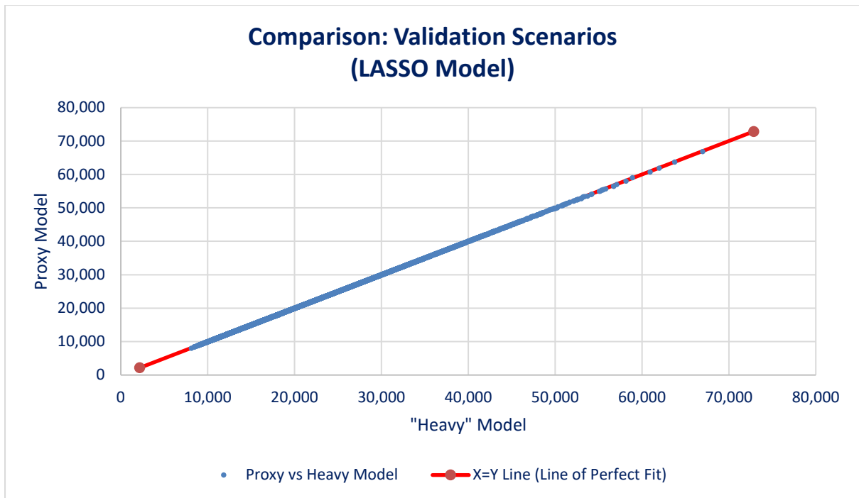
Figure 13: comparison of validation scenarios under LASSO approach
