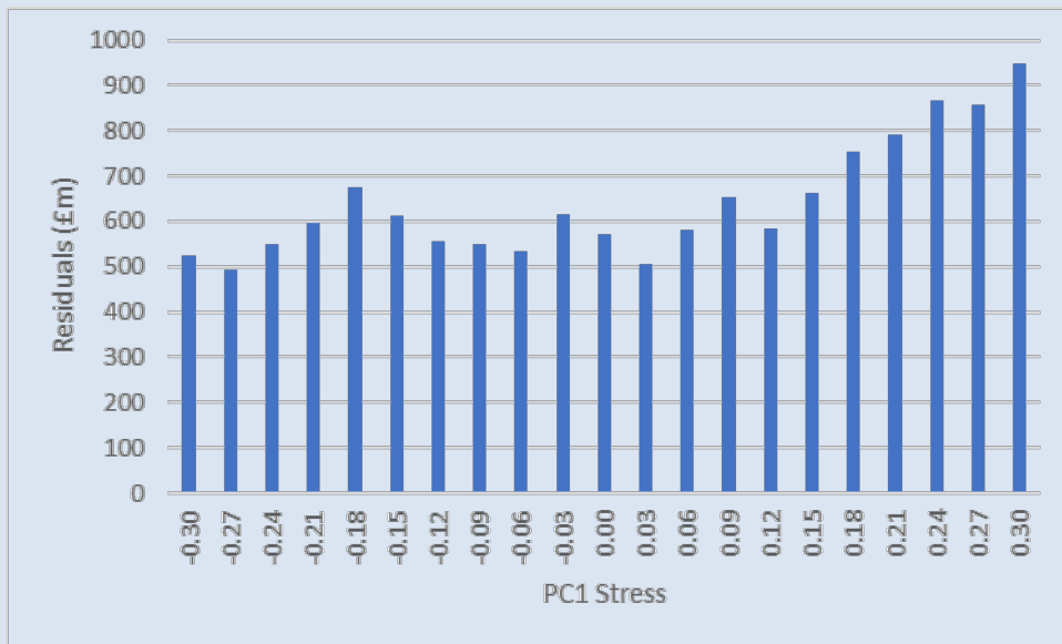
Figure 19: plotted residuals of bias test
