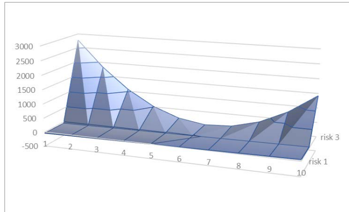
Figures 29: graphical analysis showing impact of interactions
