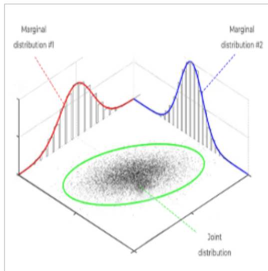
Figures 30: graphical analysis showing joint and marginal distributions
