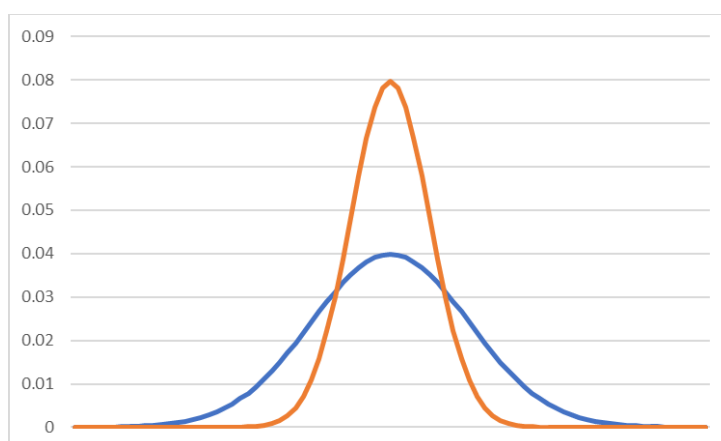
Figure 28: graphical analysis showing impact of scaling
