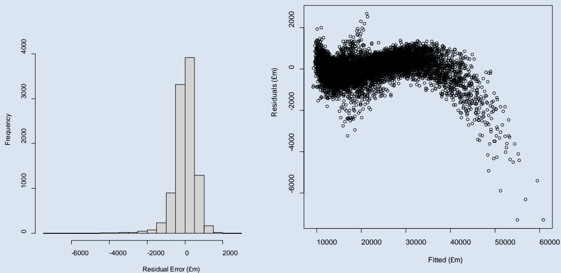
Figures 15 & 16: plotted residuals
