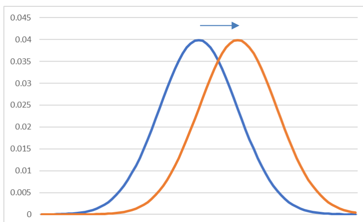
Figure 27: graphical analysis showing impact of shift
