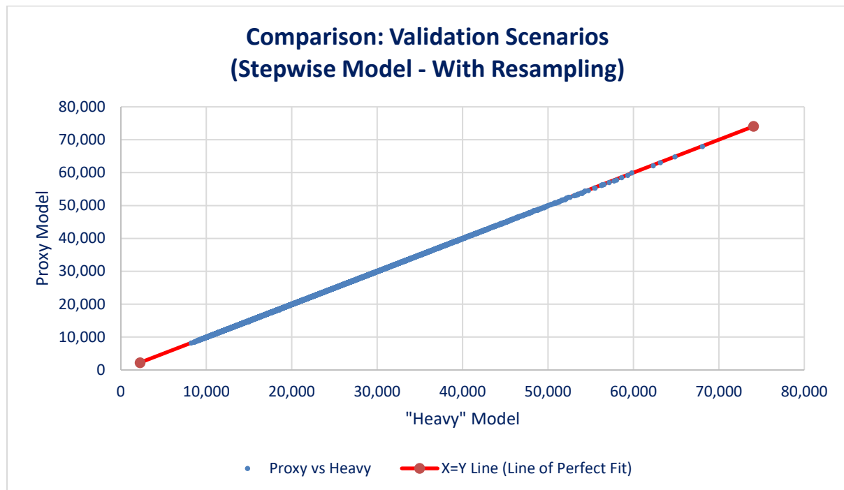
Figure 11: comparison of validation scenarios under stepwise model fitting with resampling
