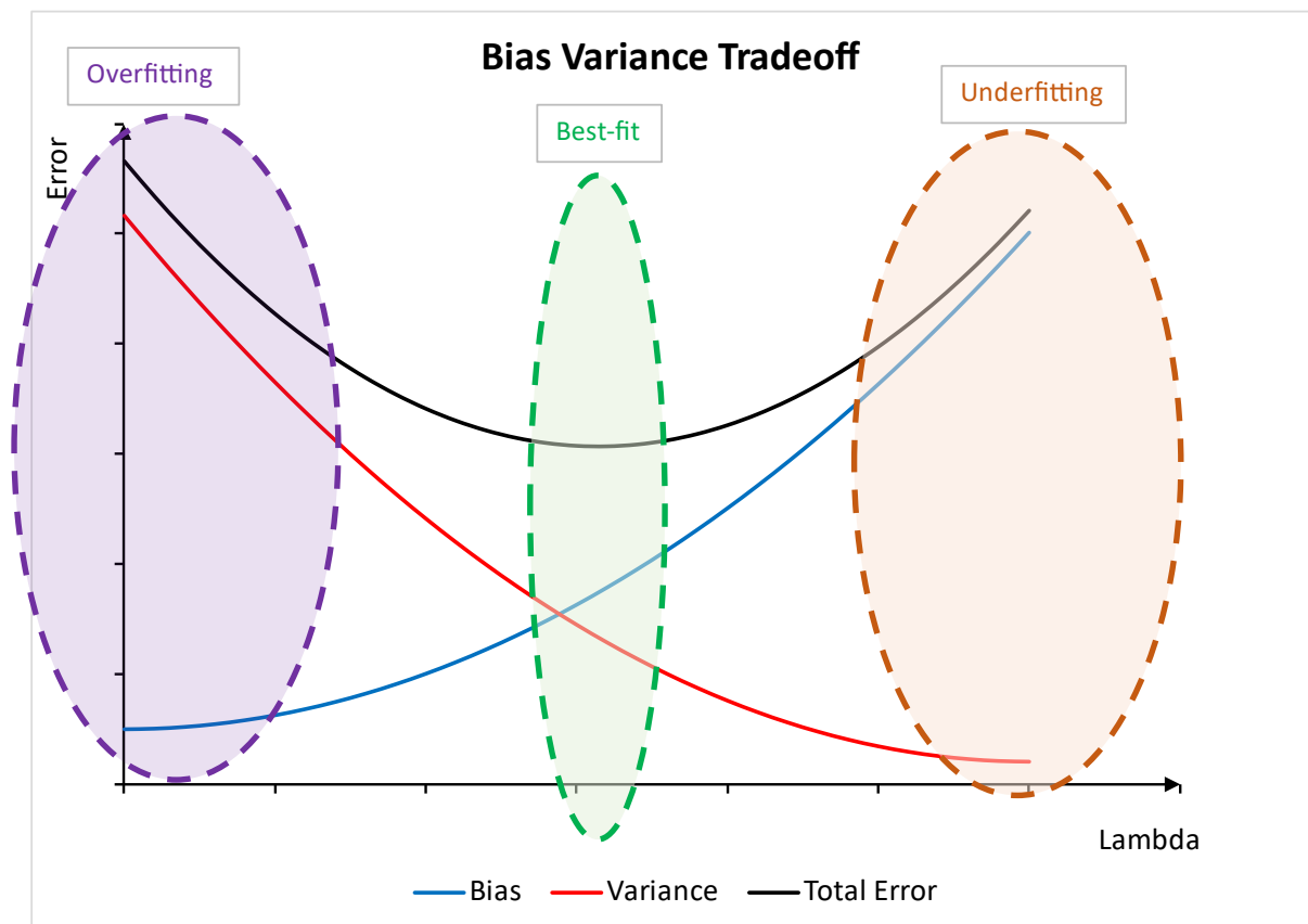
Figure 6: illustrative bias and variance trade-off
