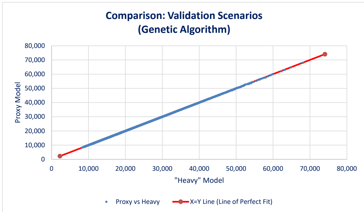
Figure 12: comparison of validation scenarios under genetic algorithm approach
